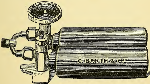
FIG. 7.—Gas bottles fixed horizontally.
